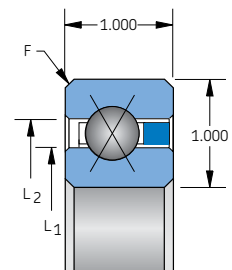
Snap-over separator 1/2" balls
