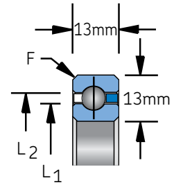
Snap-over separator 1/4" (inch) balls Conrad Assembly Type C
