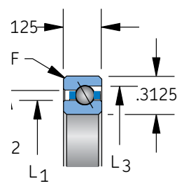
Circular pocket separator 5/32" balls
