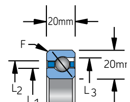
Circular pocket separator 3/8" (inch) balls Angular Contact Type A
