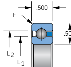
Snap-over separator 1/4" balls
