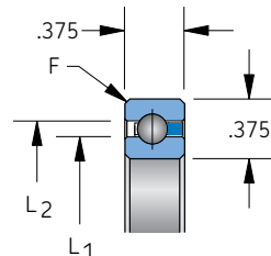
Snap-over separator 3/16" balls
