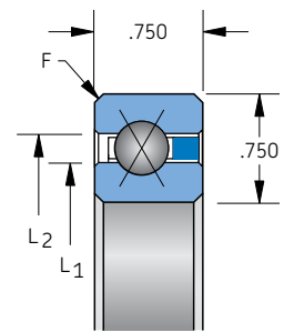
Snap-over separator 3/8" balls
