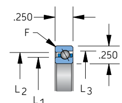
Circular pocket separator 1/8" balls
