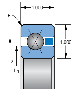
Snap-over separator 1/2" balls
