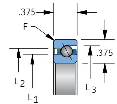
Circular pocket separator 3/16" balls
