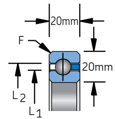
Snap-over separator 3/8" (inch) balls Conrad Assembly Type C
