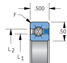
Snap-over separator 1/4" balls
